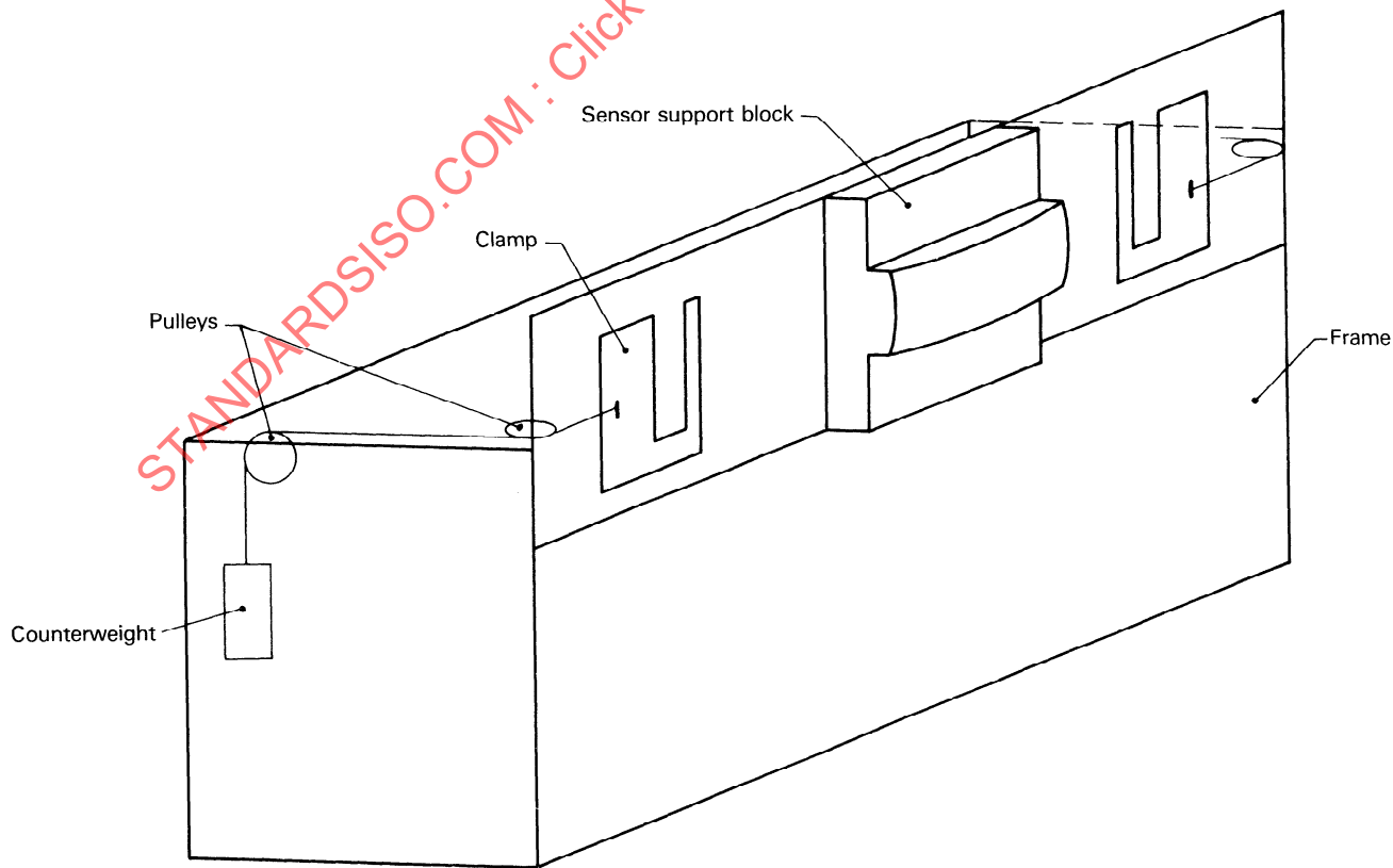
Figure 5 — Specimen support
