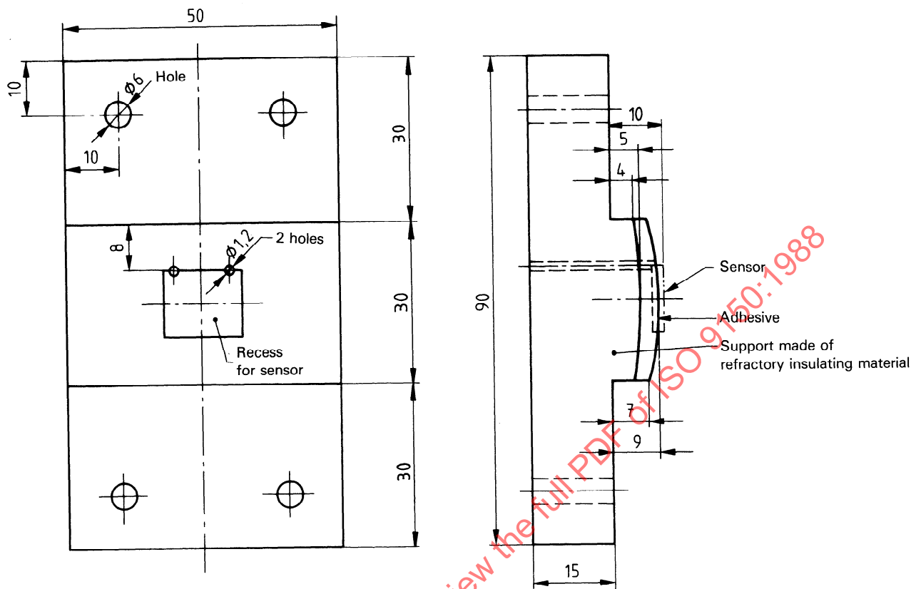
Figure 4 — Sensor support block
