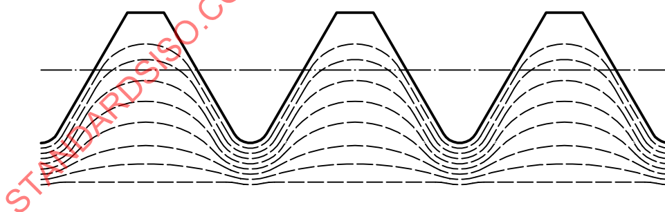
Figure 4 — Grain flow in threads (see 5.5.2)
