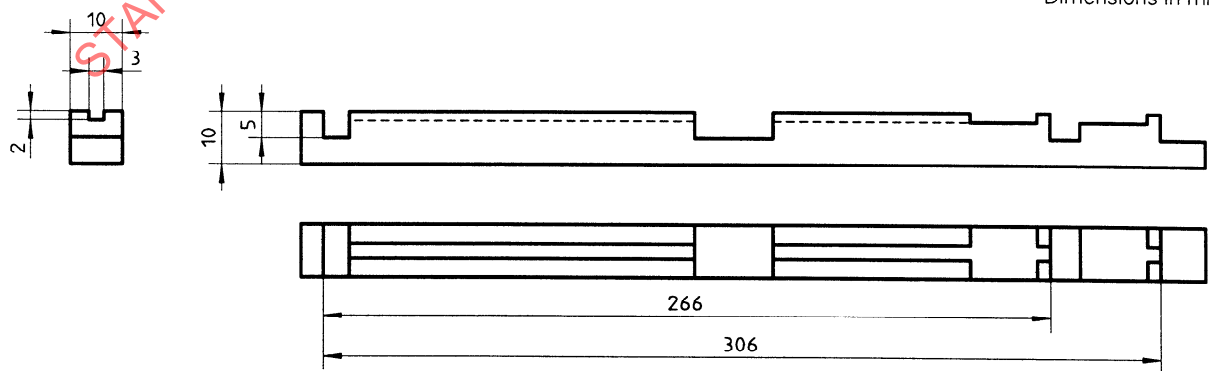
Figure A.4 — Template for cutting test specimens from impregnated roving
