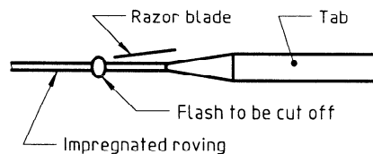
Figure A.6 — Deflashing a tab
