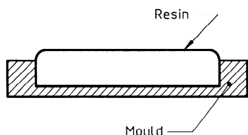
Figure A.5 — Pouring the resin
