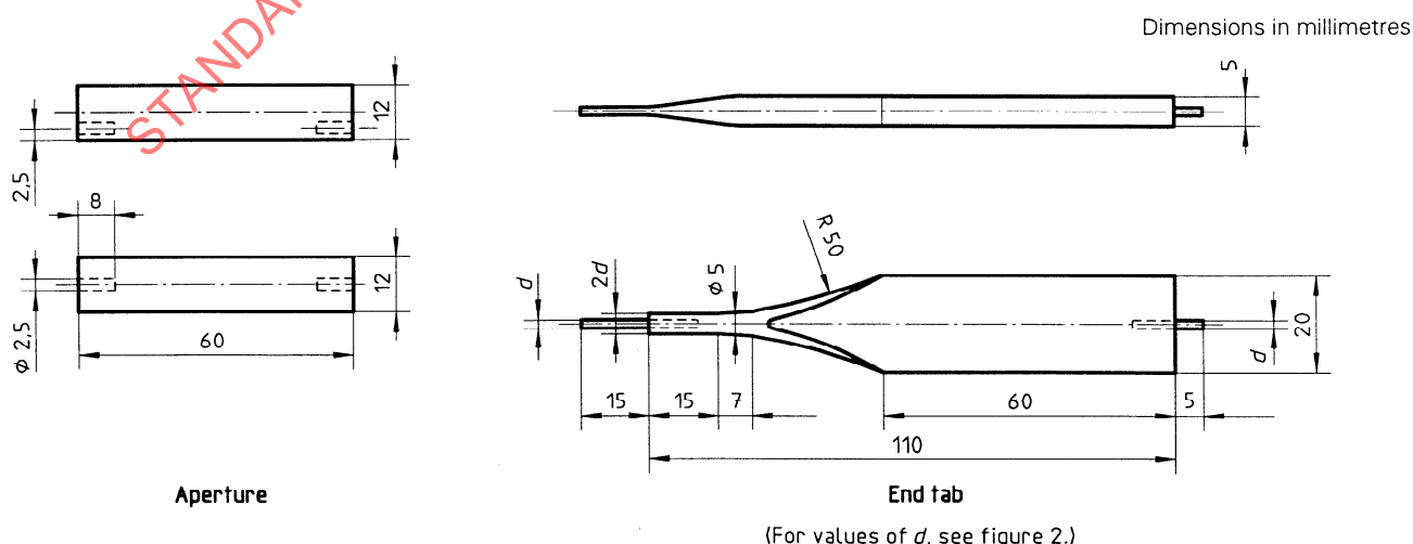
Figure A.2 — Templates for fabrication of moulds
