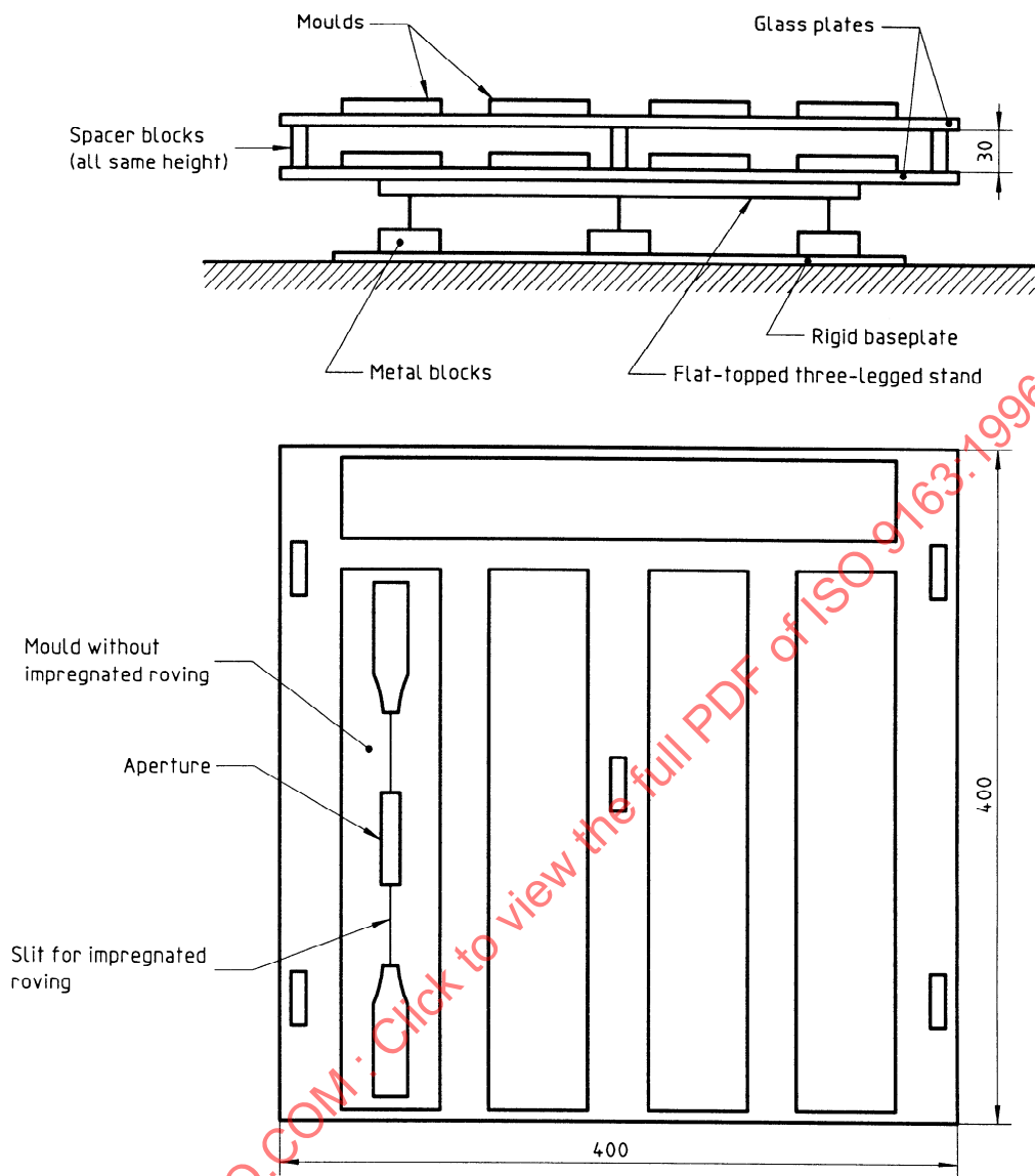
Figure A.3 — Production of end tabs
