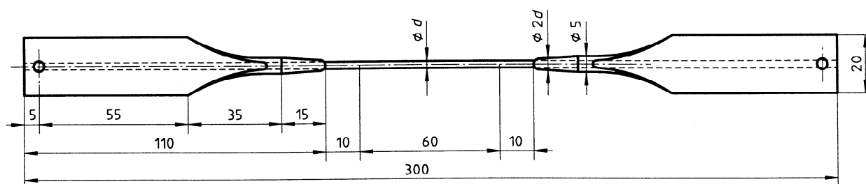
Figure 3 — Test specimen
