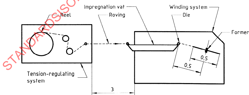
Figure 1 — General layout of impregnation apparatus
