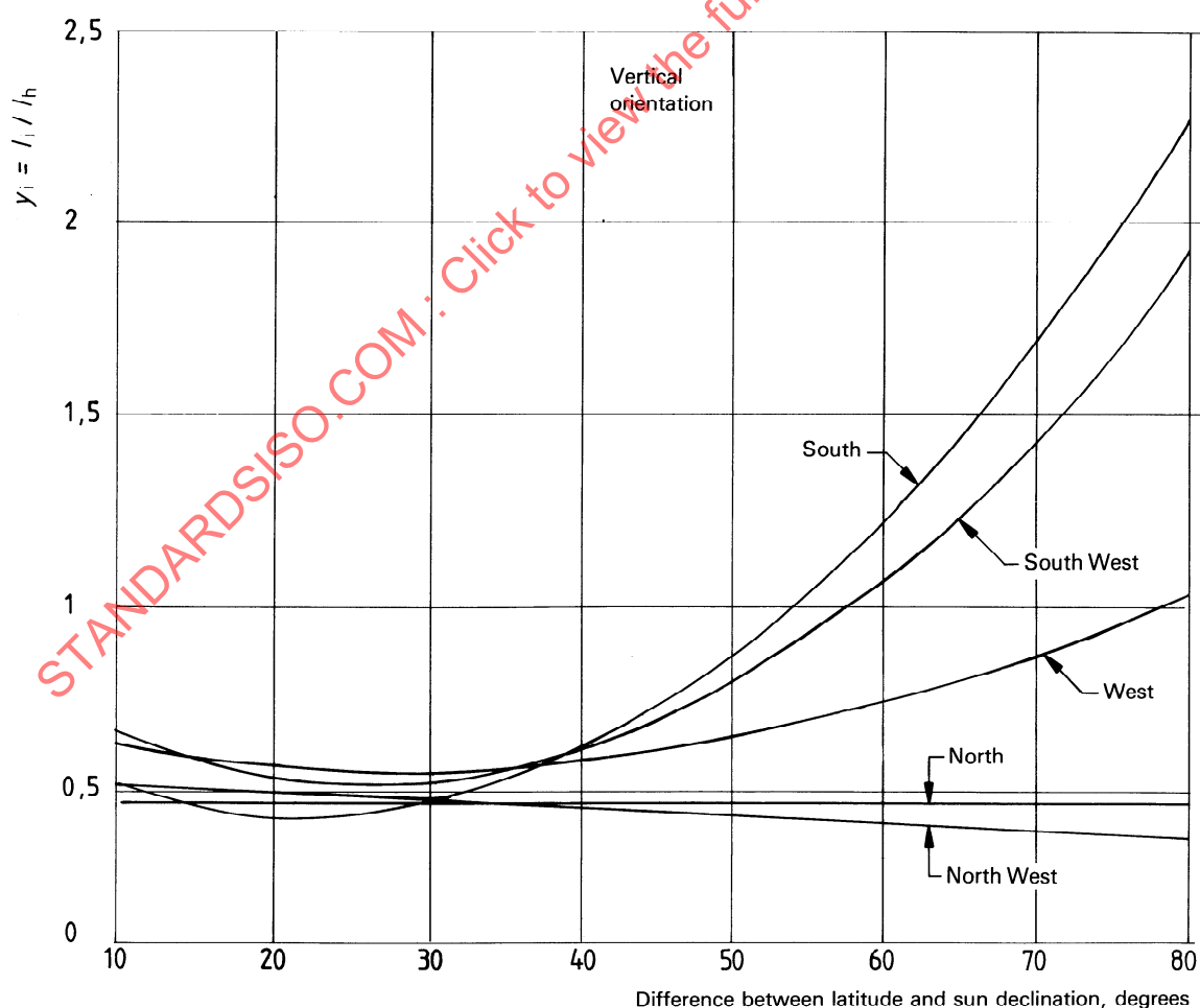
Figure D.1 — Orientation factors depending on difference of latitude and sun declination for K_h = 0,3 and R = 0,3 , obtained from the relations in table D.2
