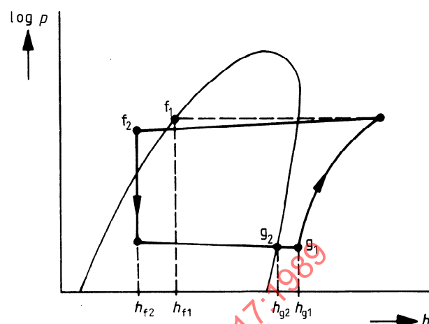
b) Log p versus h diagram
