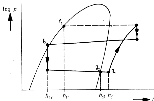
b) Log p versus h diagram
