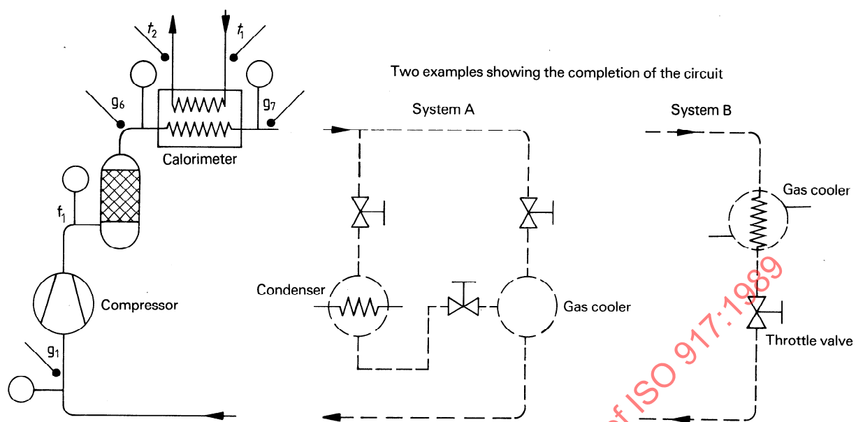
a) Circuit diagrams
