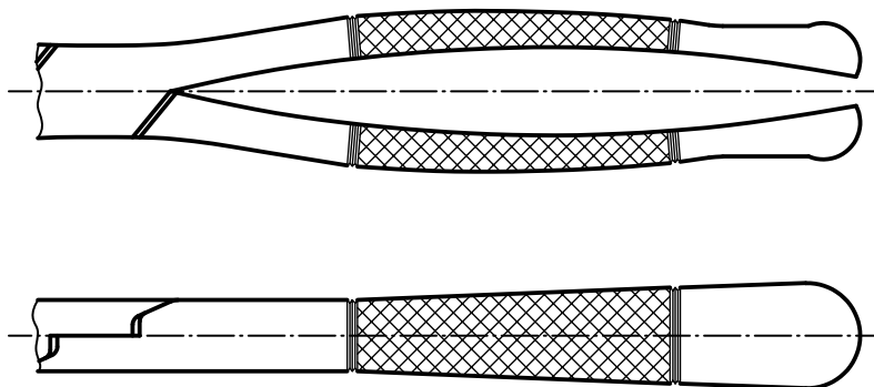
Figure 6 — Straight handle Type 1
