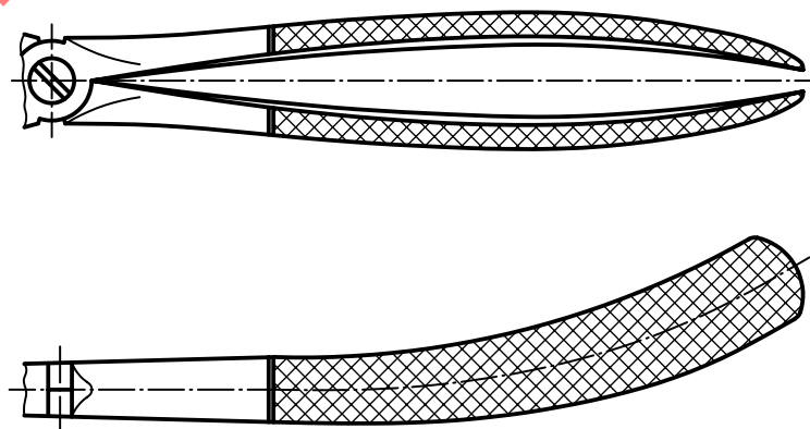
Figure 8 — Curved handle Type 1
