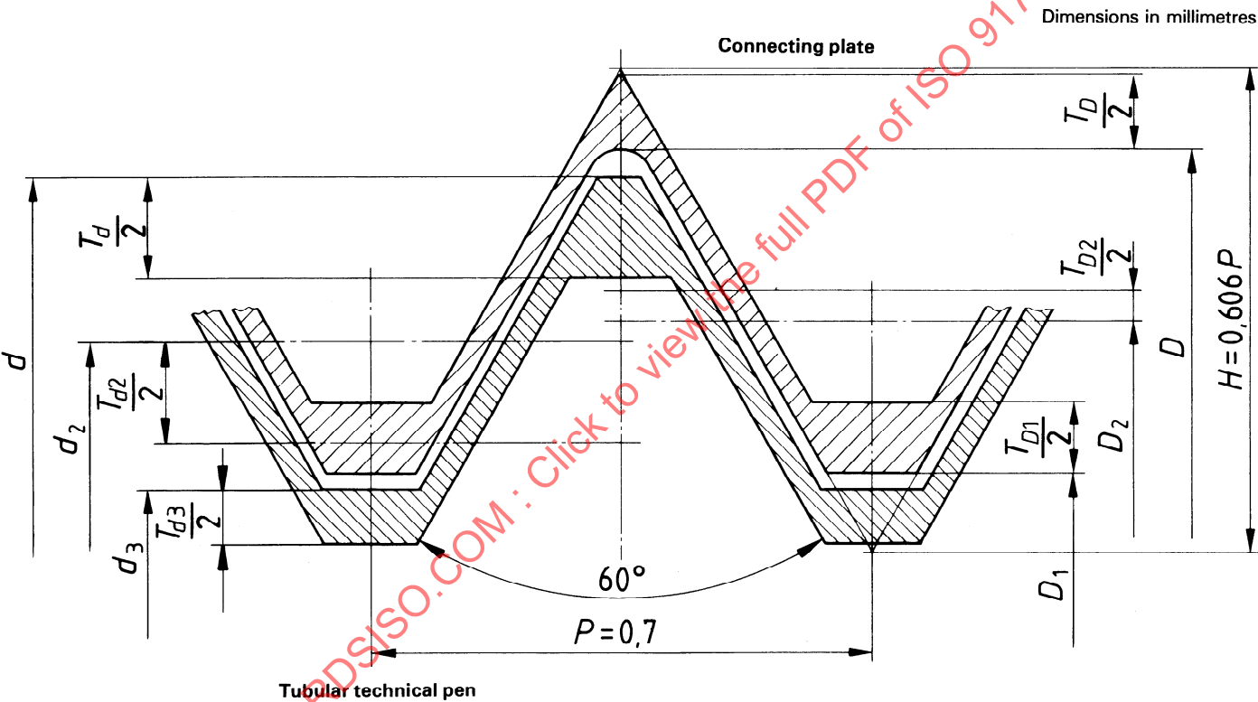
Figure 3 – Screw thread
