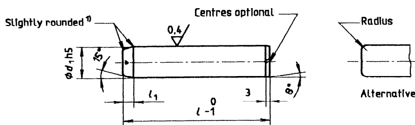
a) Type A1, straight guide pillar
