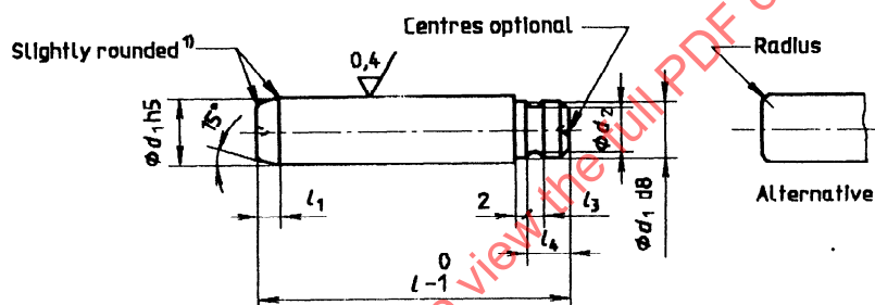
b) Type A2, straight guide pillar with end-locking and locking ring
