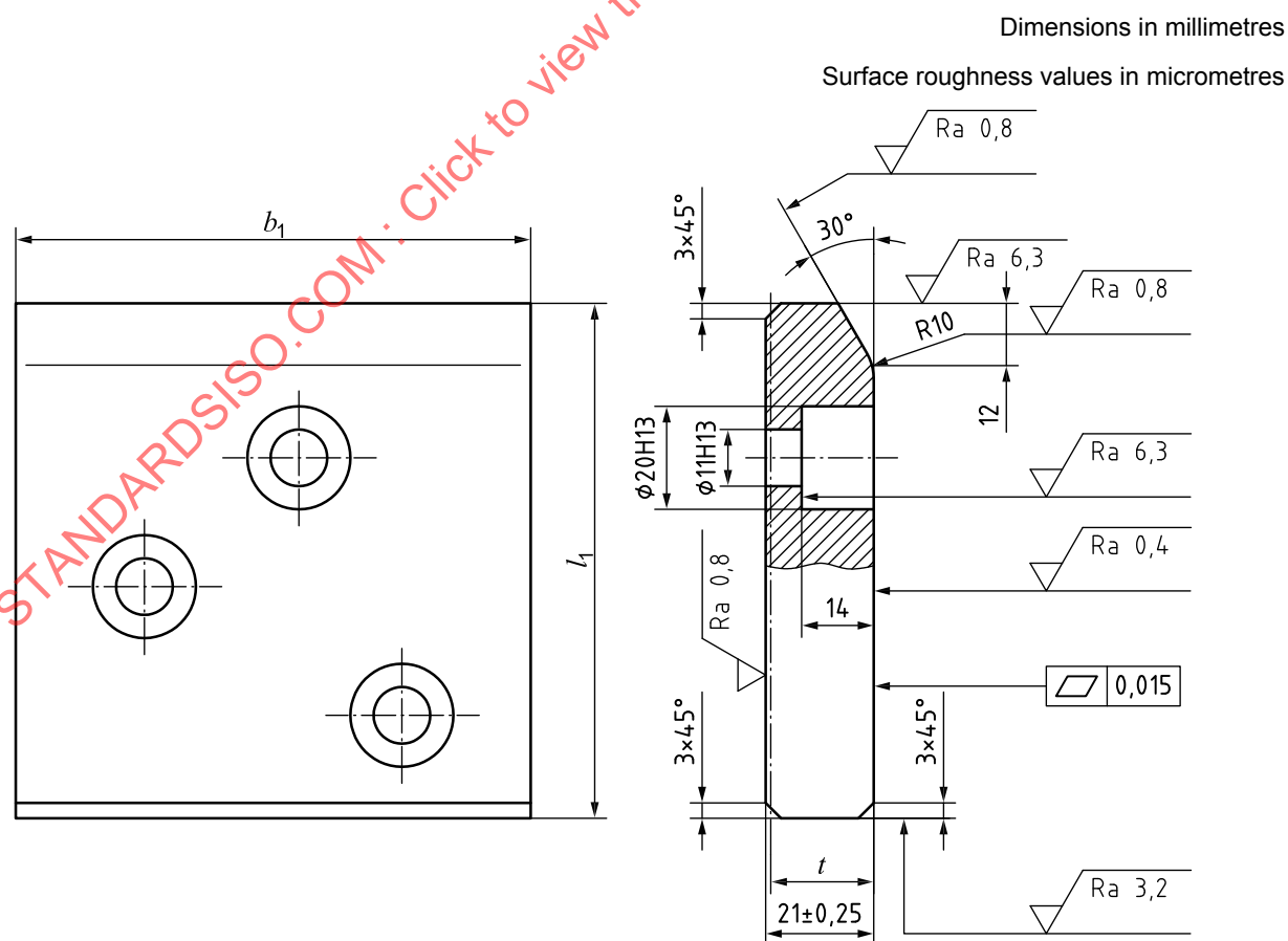
Figure 1 — Dimensions
