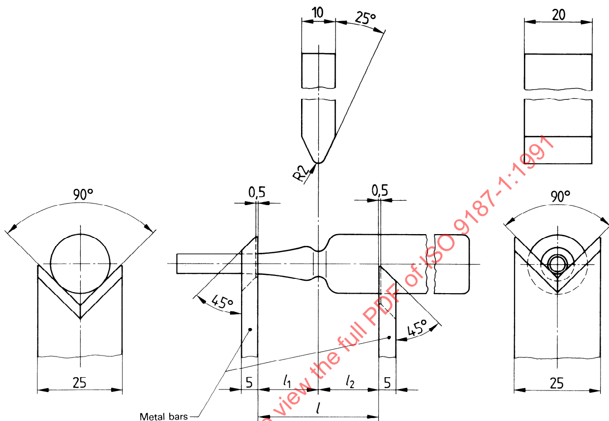
Figure 4 — Example of test set-up for determining the breaking force of ampoules
