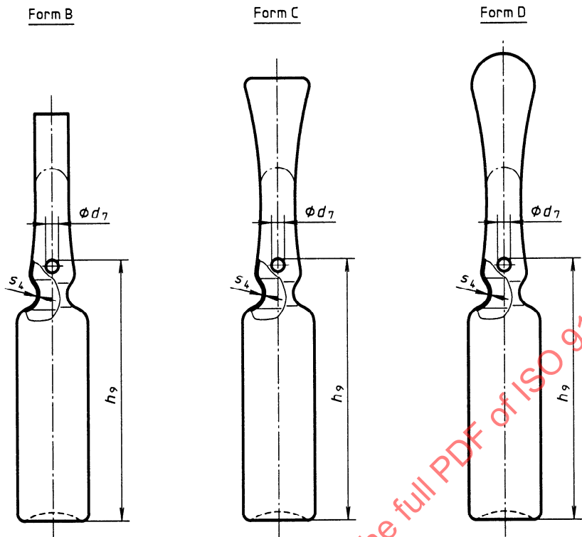
Figure 1 — Typical examples of OPC ampoules
