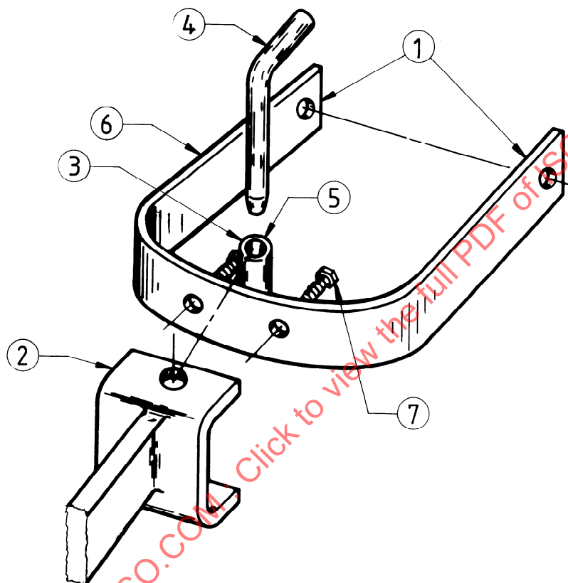
Figure 1 — Typical one-point tubular sleeve hitch
