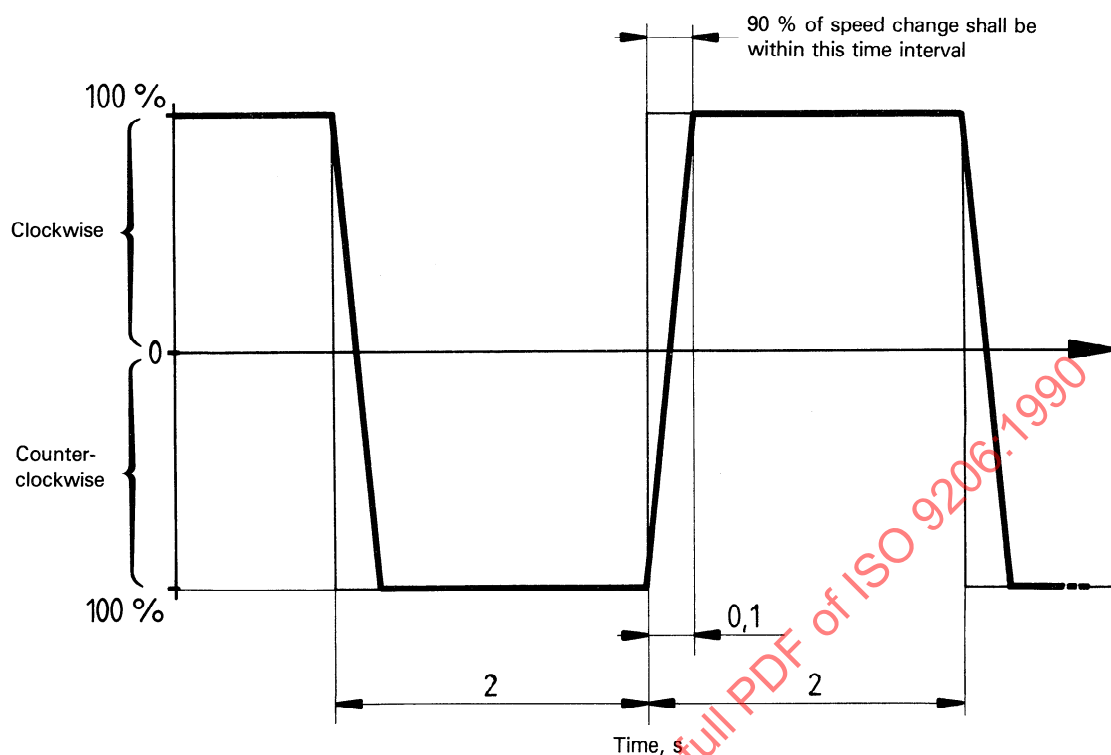
Figure 2 — Square wave speed cycle test
