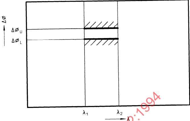
Figure 8 — Phase-changing function
