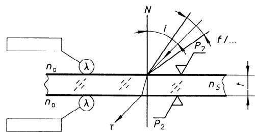
Figure A.4 — Transmittance, conical, oblique incidence
