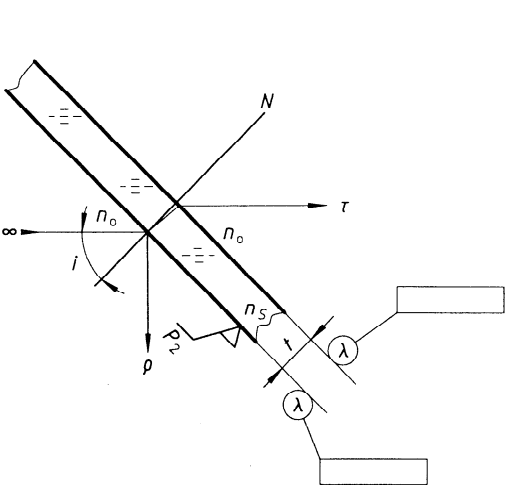
Figure A.5 — Beamsplitter, plate
