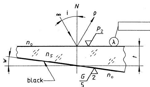
Figure A.1 — Reflectance, collimated beam
