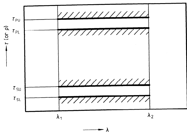
Figure 7 — Polarizing function
