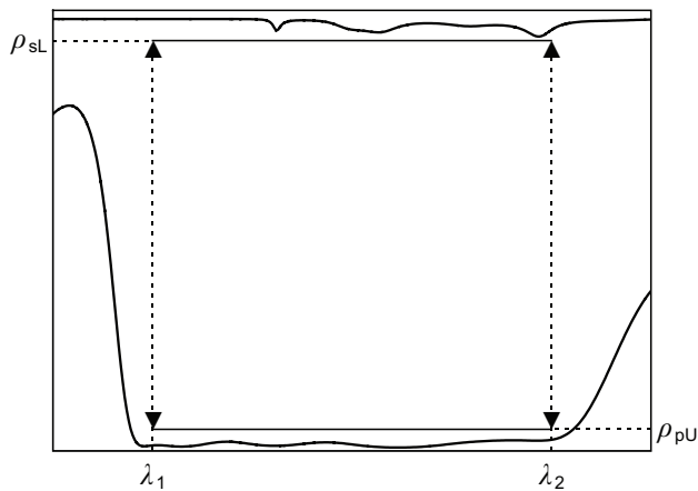
Figure 9 — Polarizing function
