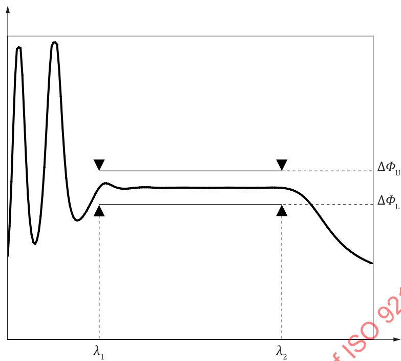
Figure 10 — Phase changing function
