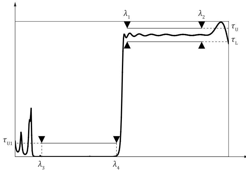
Figure 7 — Selecting function of long pass type
