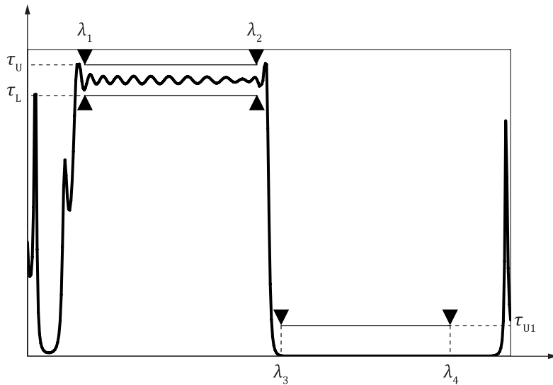
Figure 8 — Selecting function of short pass type
