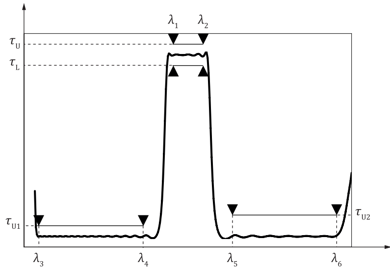
Figure 5 — Filtering function of bandpass type
