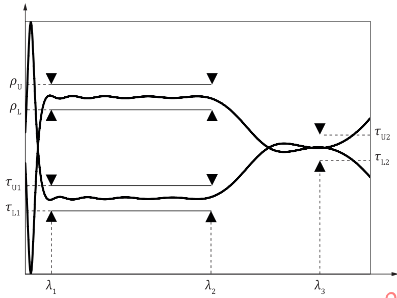
Figure 3 — Beam splitting function
