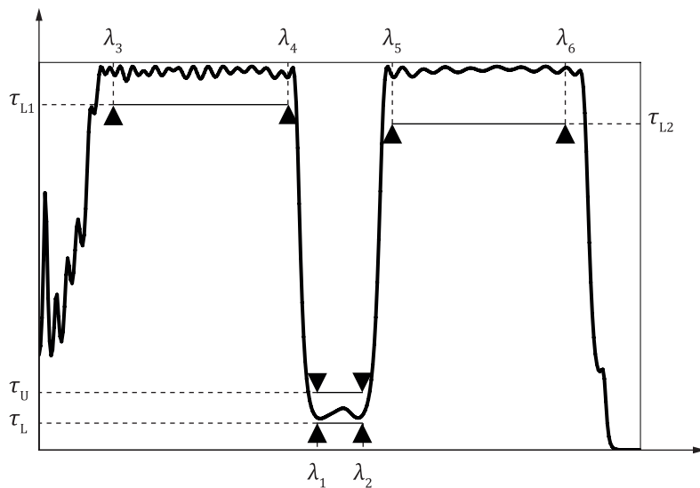
Figure 6 — Filtering function of band rejection type
