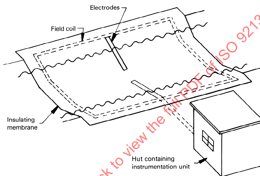
Figure 1 — Buried coil configuration
