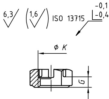
a) Form of size code 050
