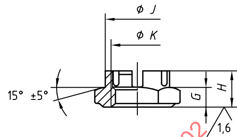
b) Form of size code 060
