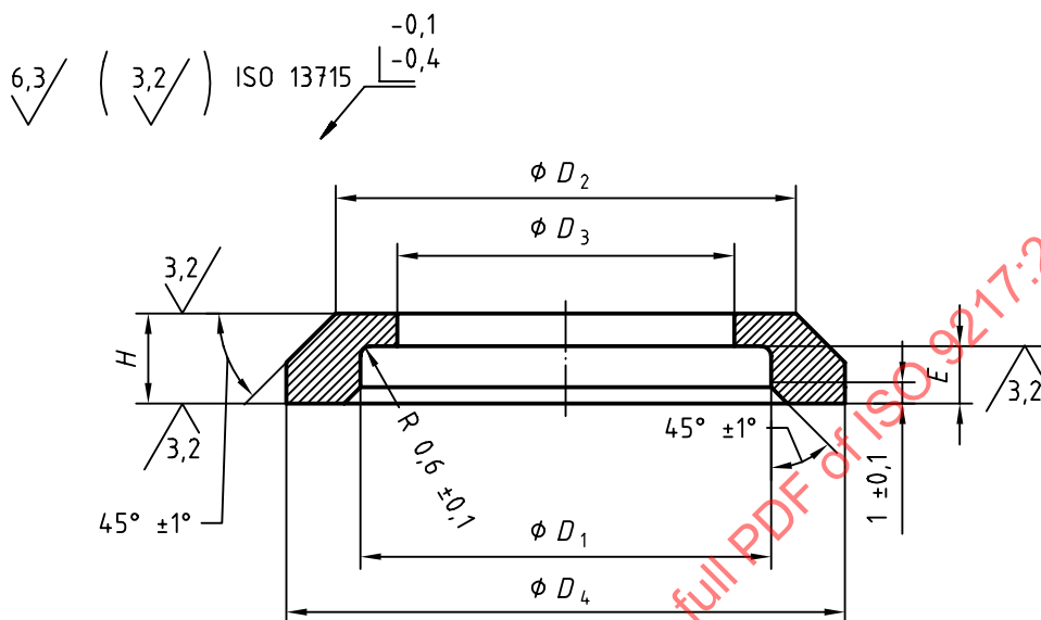
Figure 1 — Chamfered washer
