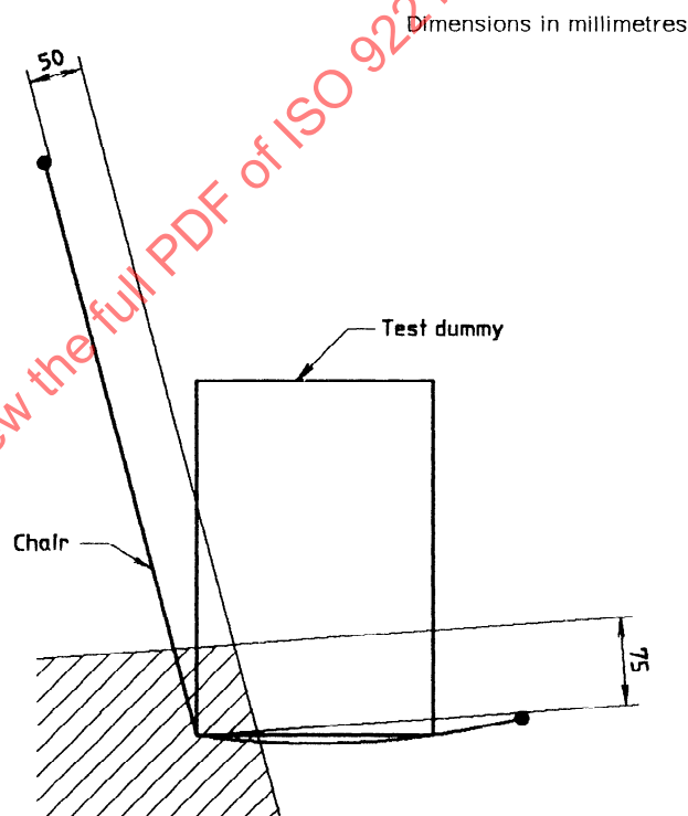
Figure 1 — Location of harness attachment points
