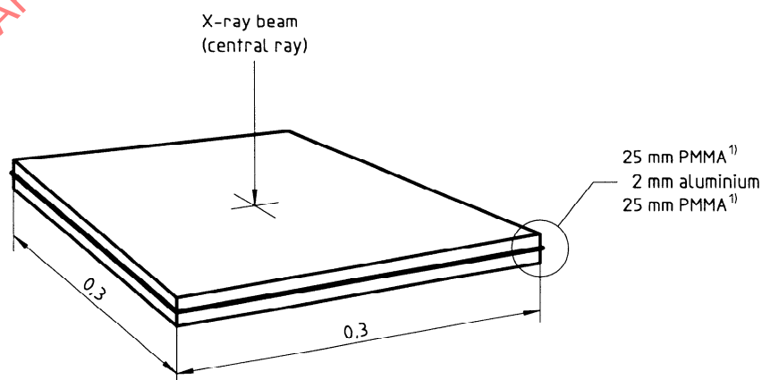
Figure 4 — Phantom for technique I
