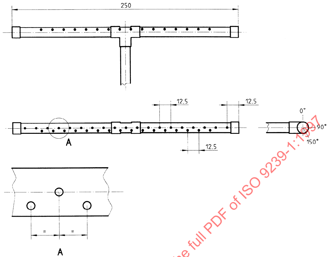
Figure 7 — Pilot burner
