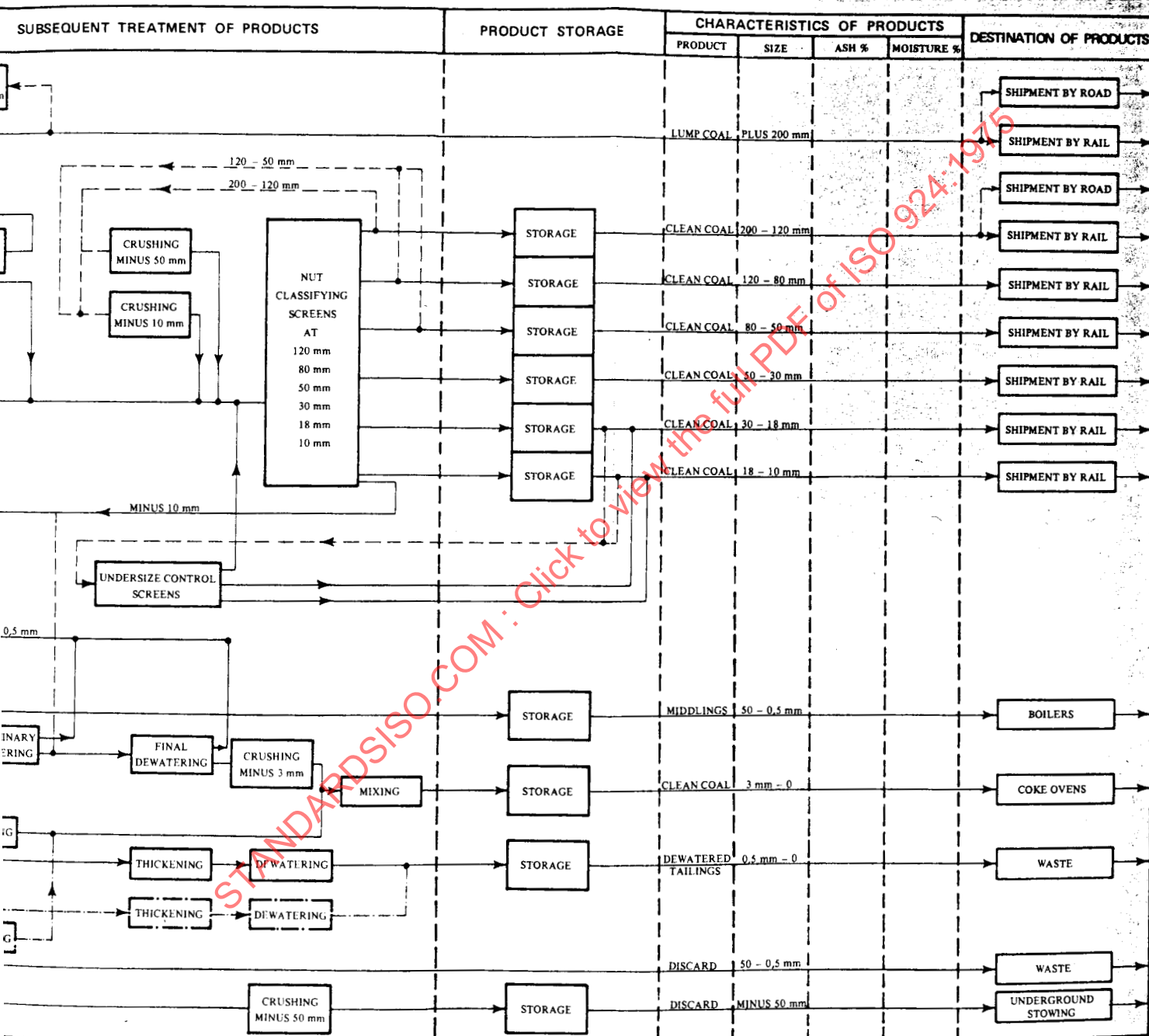
Sample of process flowsheet
