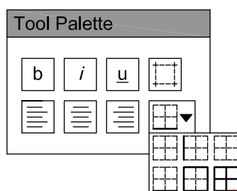
Figure 40 — Cascading tool palette
