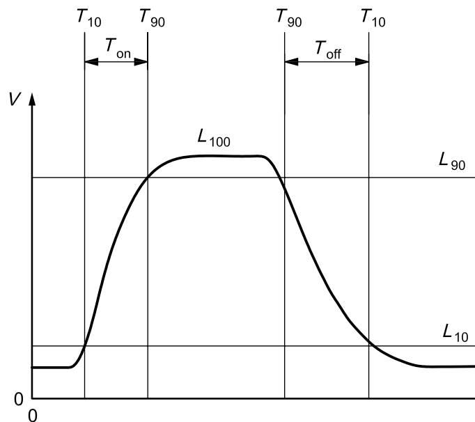
Figure 52 — Example of response times
