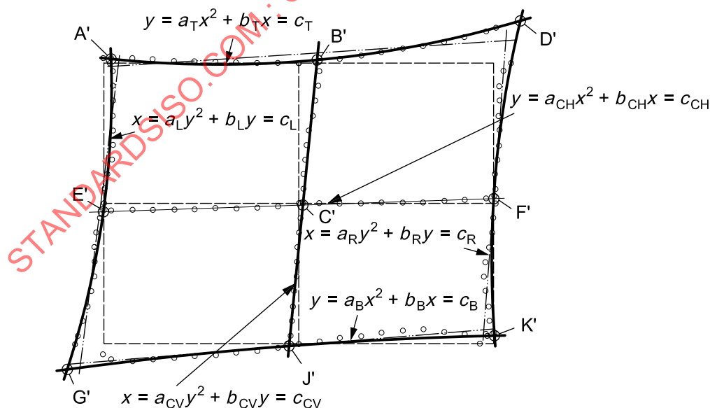
Figure 69 — Pincushion distortion analysis
