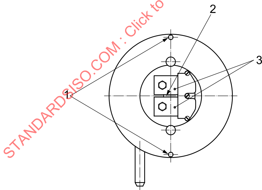
Figure 2 — Stray light elimination tube
