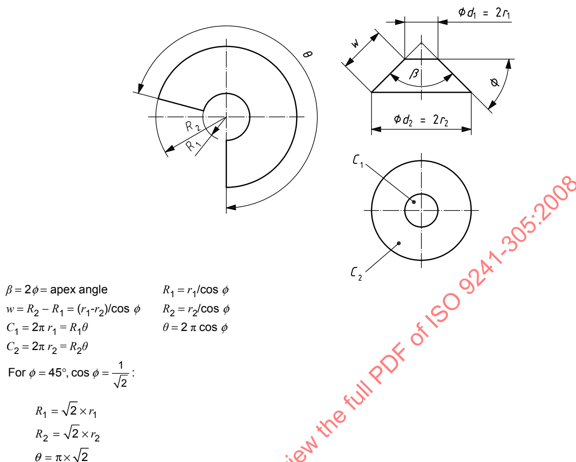
Figure 1 — Pattern for veiling glare frustum
