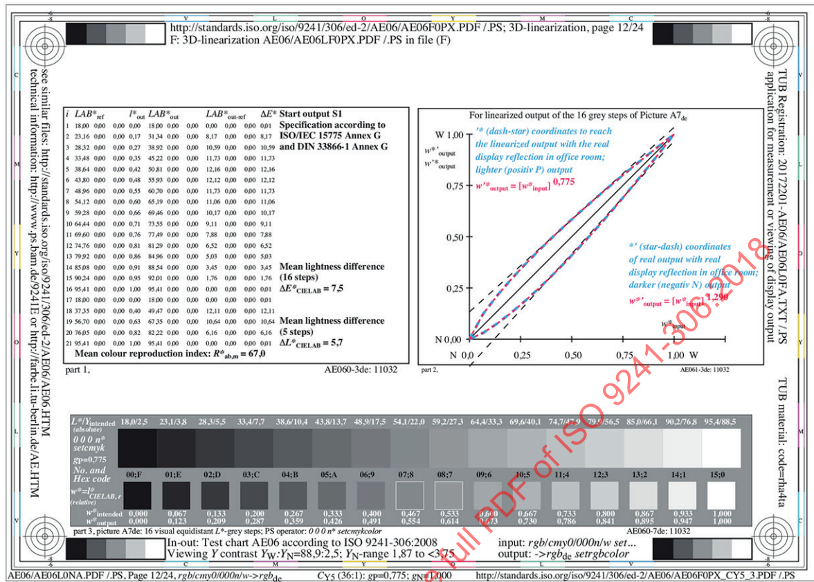
Figure D.12 — Input – output relation for output of achromatic test chart AE06 for contrast step C_{Y5}
