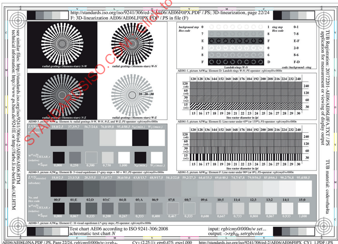
Figure D.11 — Achromatic output of test chart AE06 for contrast step C_{Y1} ( g_p = 0,47 )
