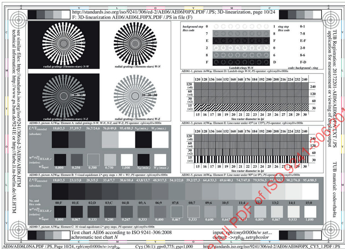
Figure D.10 — Achromatic output of test chart AE06 for contrast step C_{Y5} ( g_p = 0,77 )
