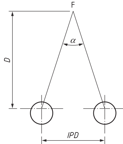
Figure C.3 — Convergence angle
