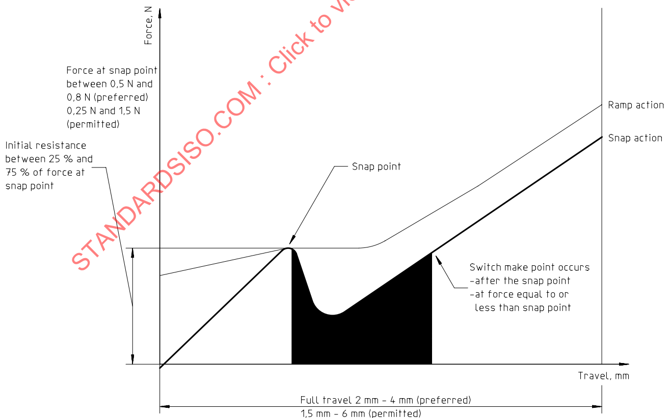
Figure 8 — Relationship between key displacement and key force
