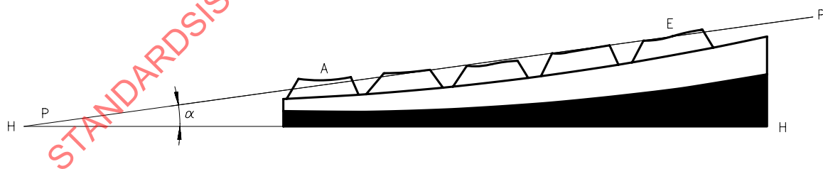
Figure 5 — Keyboard slope
