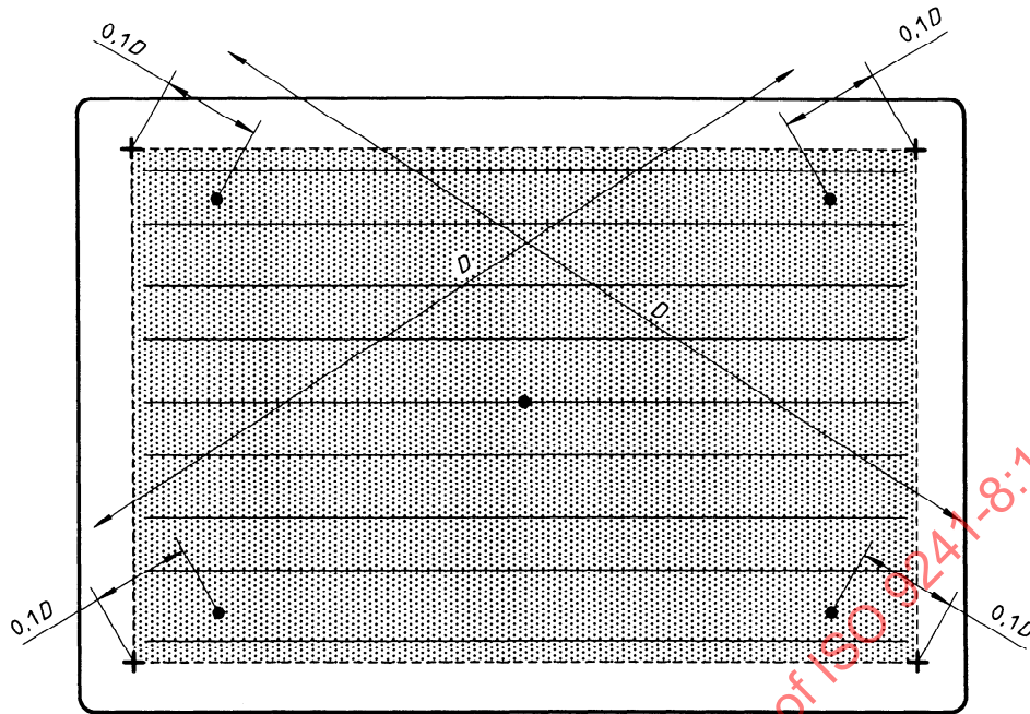
Figure 8 – Measurement locations
