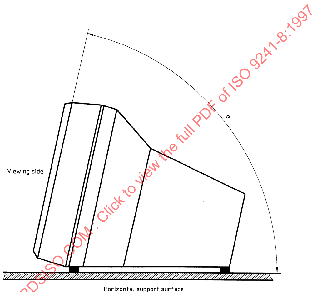
Figure 7 — Screen tilt angle
