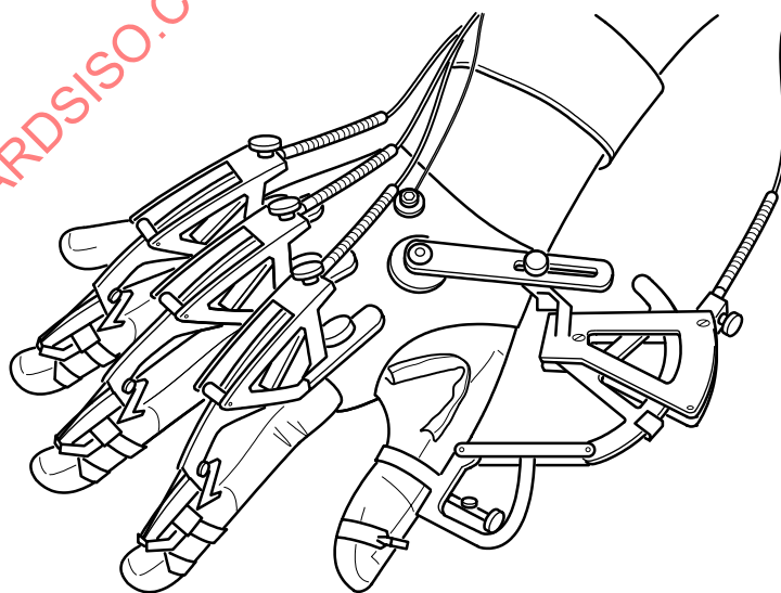
Figure B.6 — Hand-based haptic device
