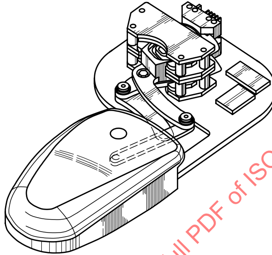
Figure B.7 — Mouse that provides force feedback
