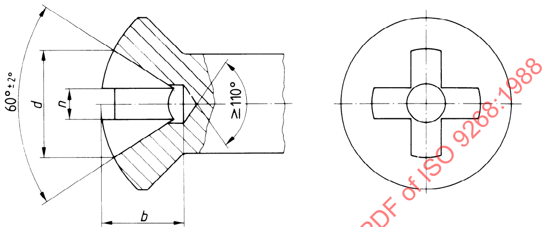
Figure 7 — Cross-recessed drive connection
