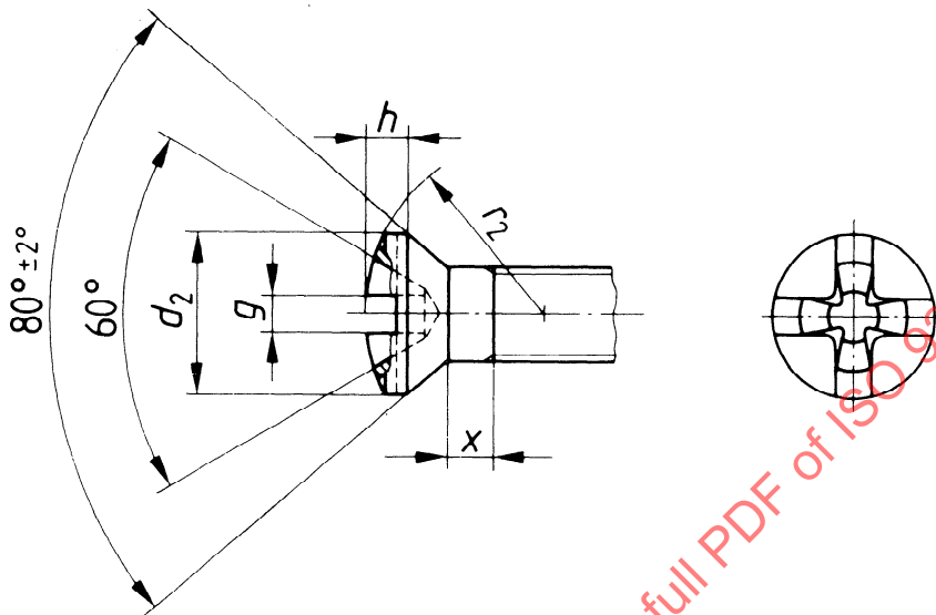
Figure 3 — Screw head with combined cruciate-slot and cross-recessed drive connection
