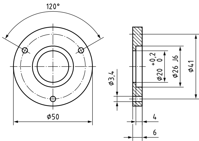
Figure B.4 — Mounding support for ball bearing
