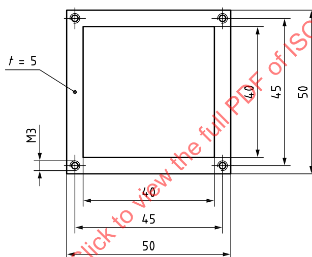
Figure A.1 — Clamp specimen holder — Bottom part
