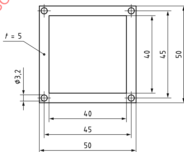
Figure A.2 — Clamp specimen holder — Top part
