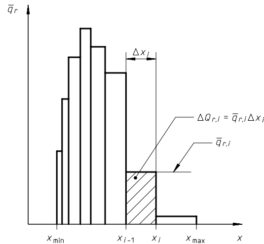
Figure 2 — Histogram of a density distribution function q_r(x)
