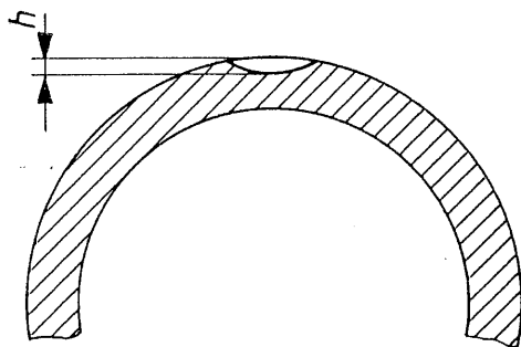
c) Arc notch
