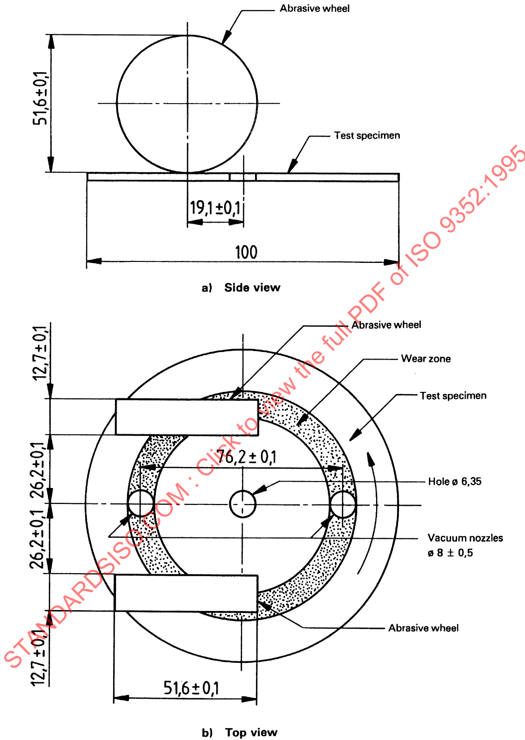
Figure 1 — Diagrammatic arrangement of apparatus
