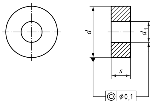
Figure 8 — Round inserts
