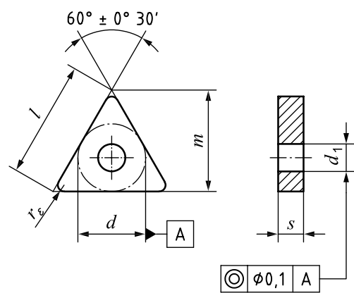
Figure 3 — Triangular inserts
