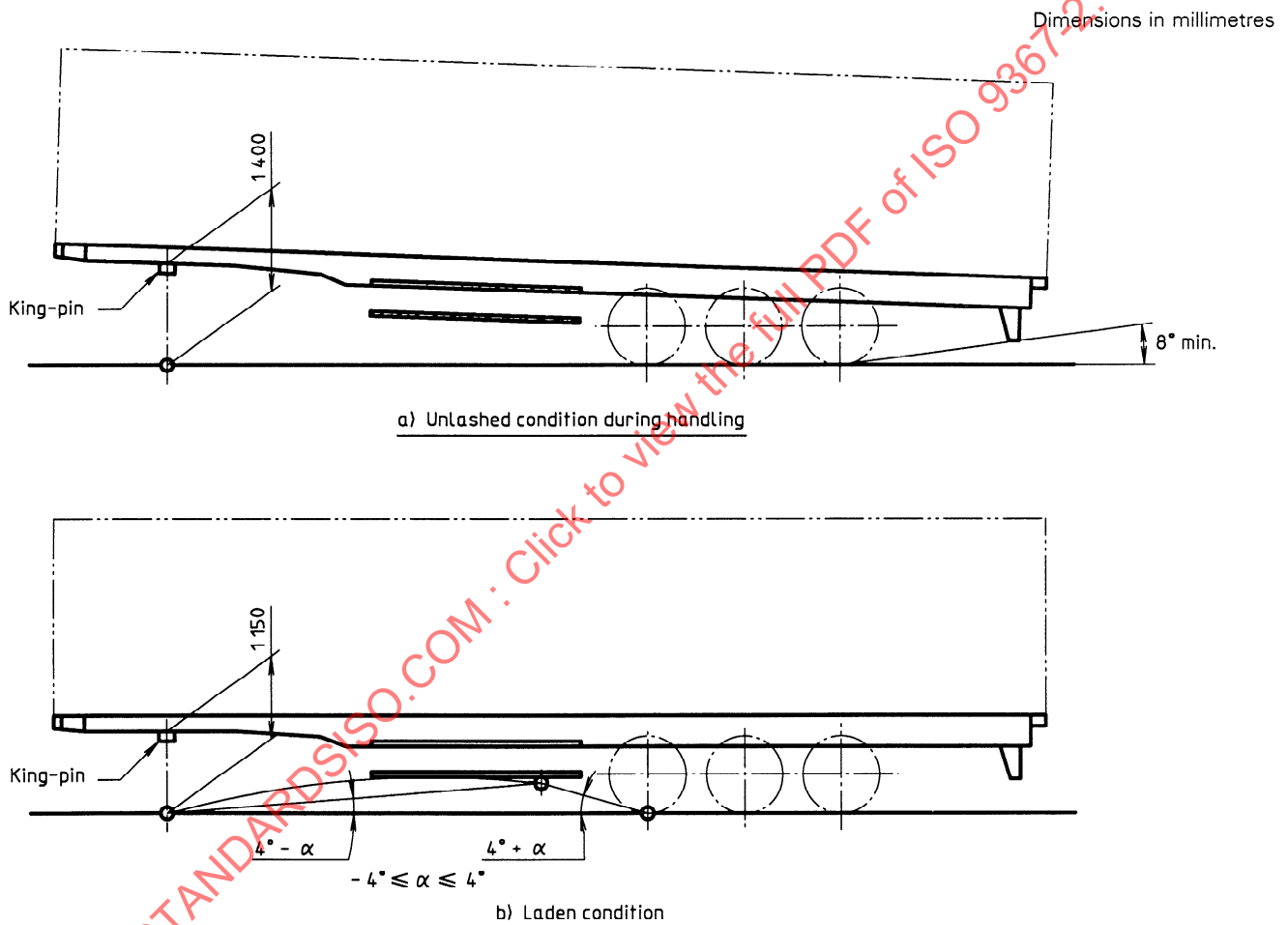
Figure 10 — Clearance gauge
