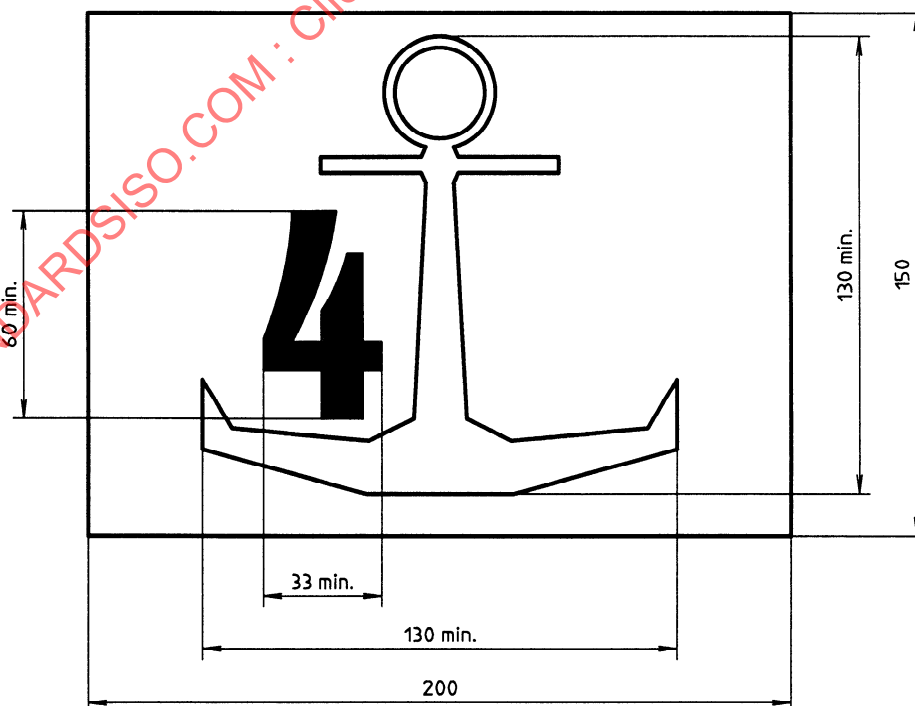
Figure 9 — Information plate
