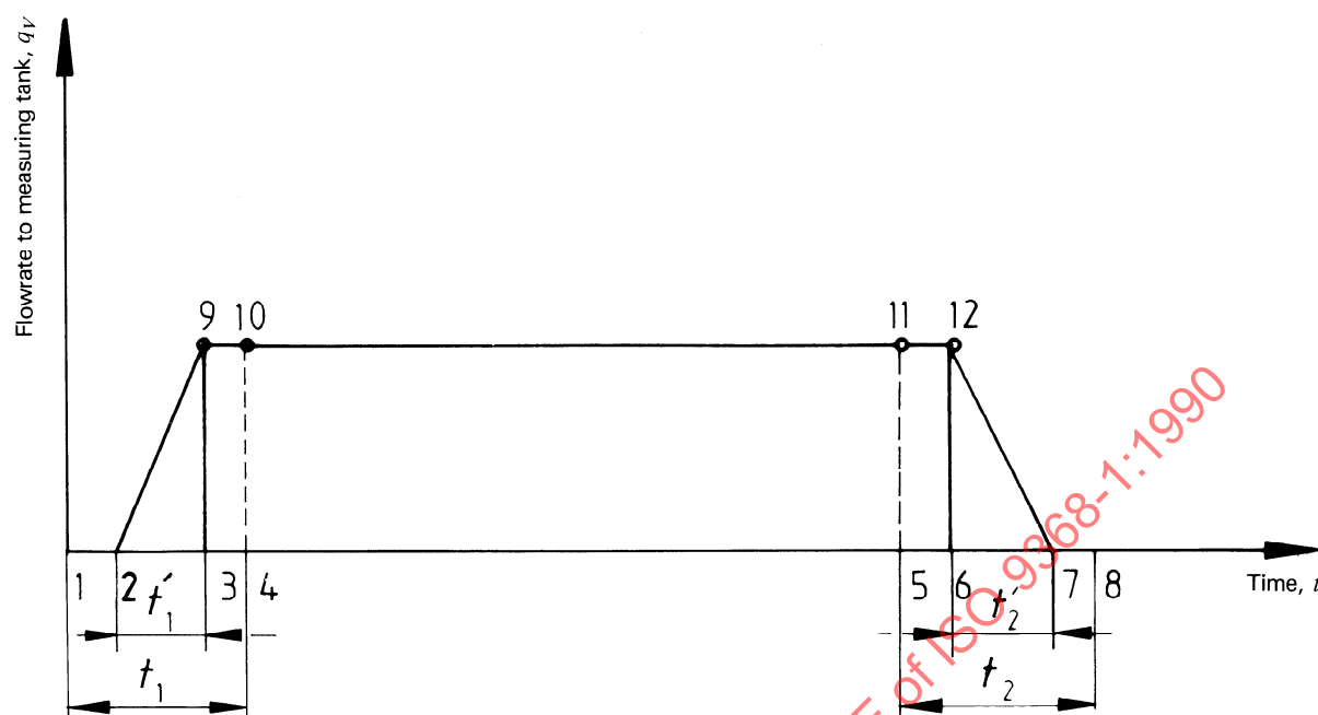
Figure B.1 — Graph of the filling process for the measuring tank
