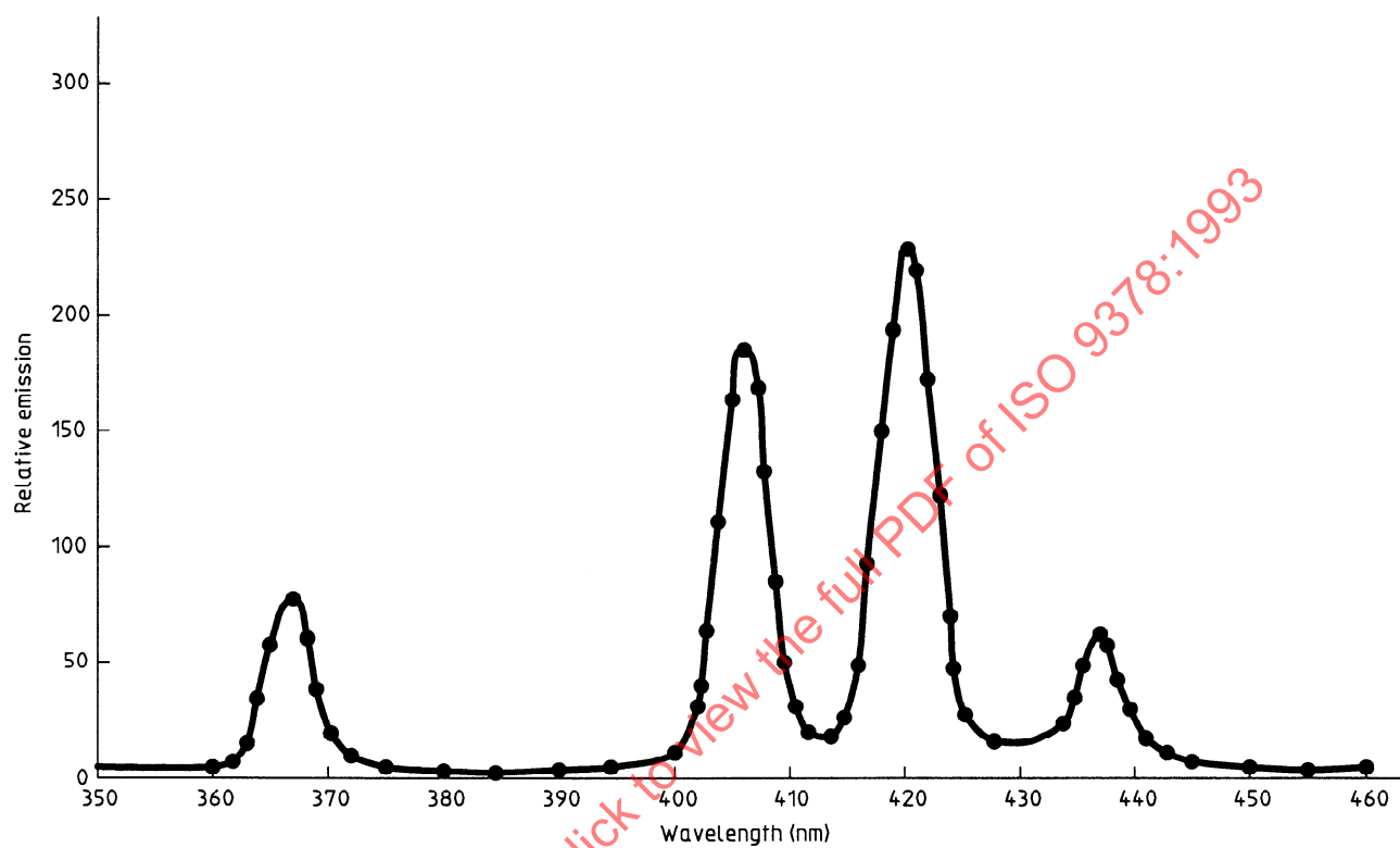
Figure A.1 — Typical spectral distribution of gallium-iodide-doped mercury lamp
