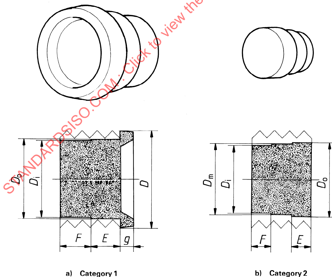
Figure 26 — Plugs
