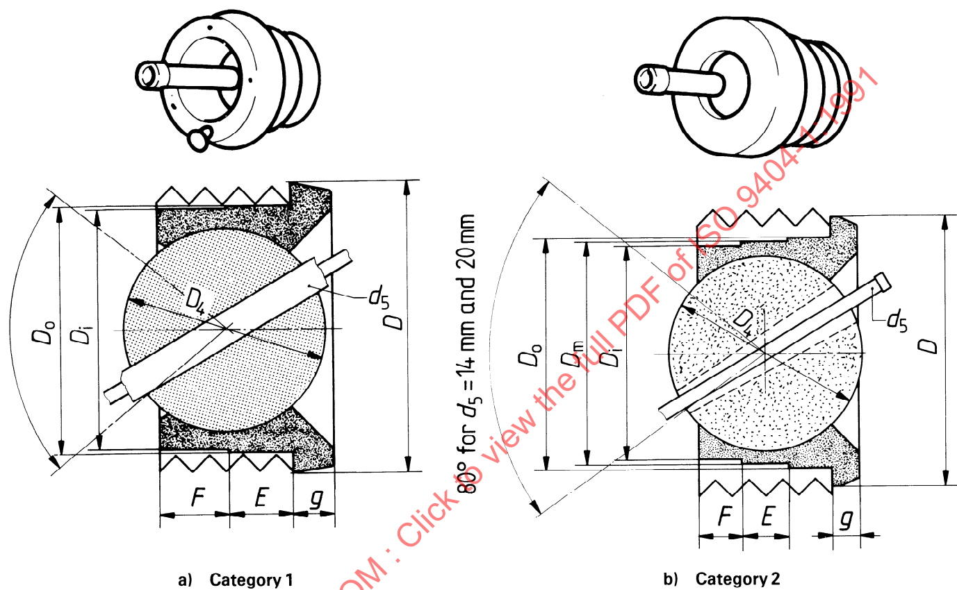
Figure 25 — Sphere units
