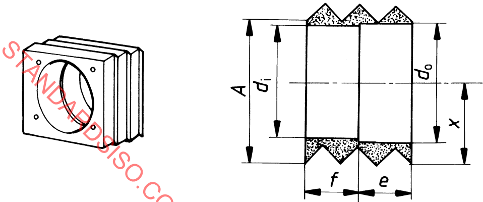
Figure 8 — Aperture brick for circular units
