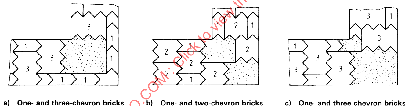
Figure 18 — Examples of corner construction with corner bricks and plain bricks
