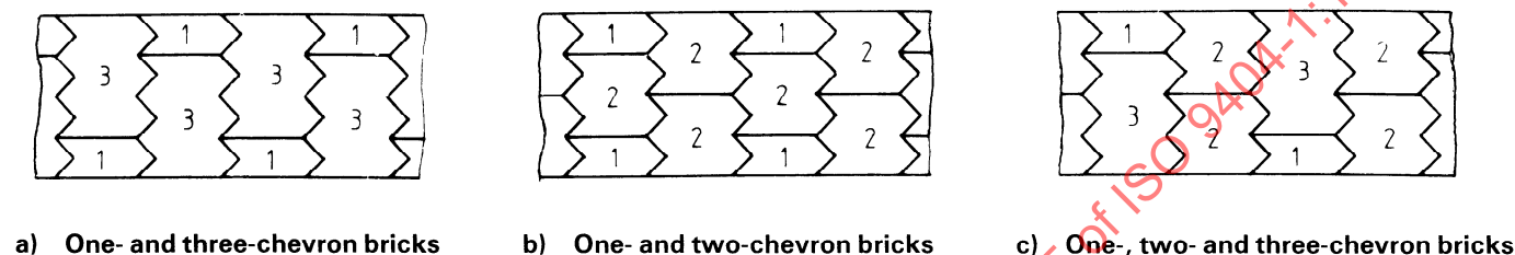
Figure 17 — Examples of wall construction with plain bricks
