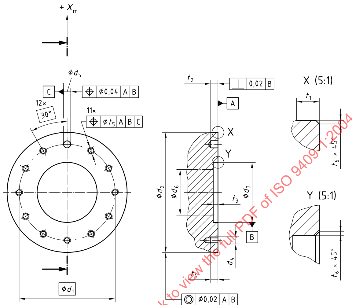
Figure 2 — Design according to Table 1, position 10
