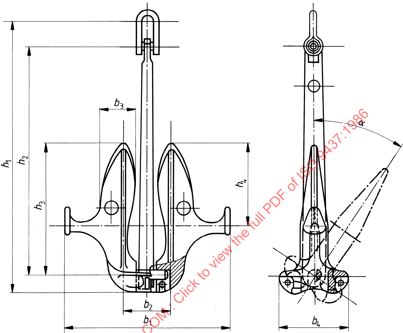
Figure 1 — Matrossov anchor, type A
