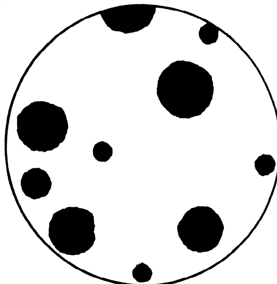
FIGURE 4 — Reference diagrams 1) for the graphite size (Forms I and VI — Distribution A) (magnification \times 100 ) — Reference Nos. 3 and 4
