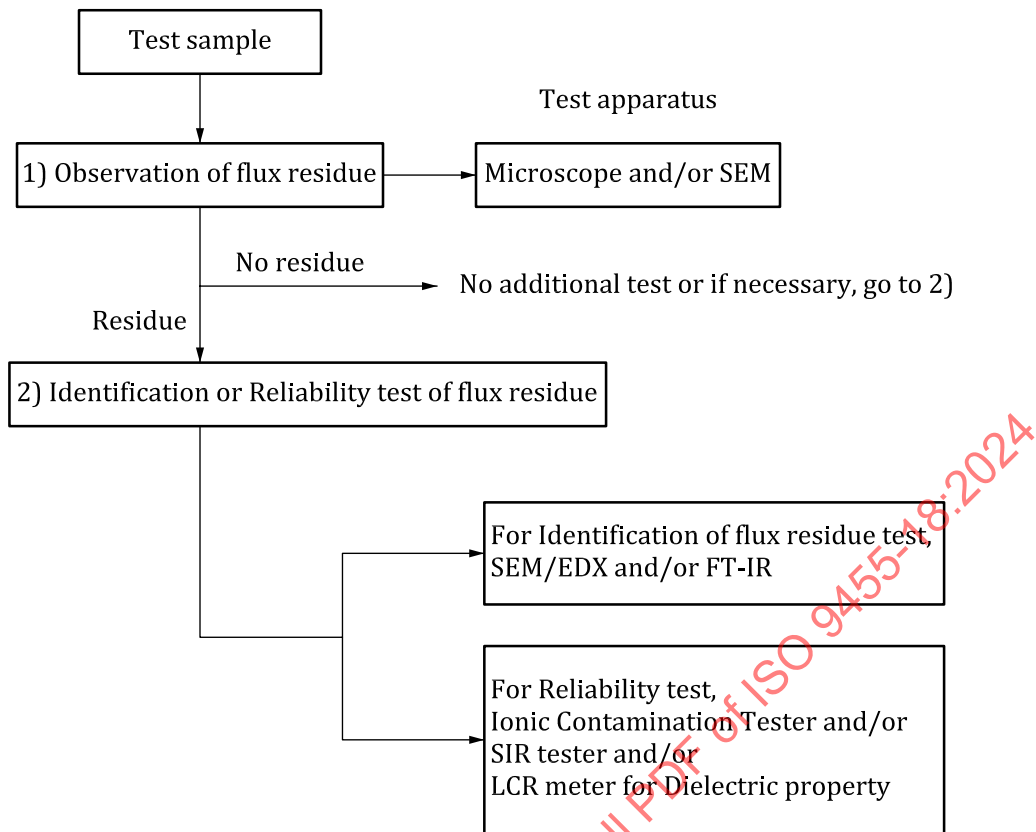
Figure 1 — Flowchart of test methods of cleanliness of the soldered printed circuit assemblies before and/or after cleaning
