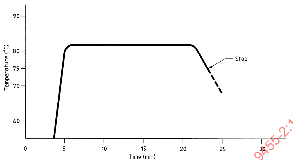
Figure 2 — Typical distillation curve
