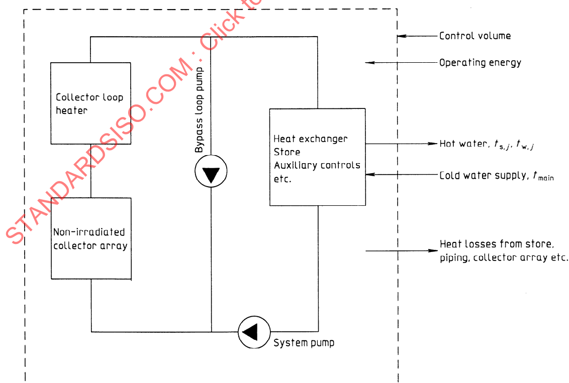
Figure 1 — Schematic representation of experimental apparatus for indoor test with non-irradiated collector array
