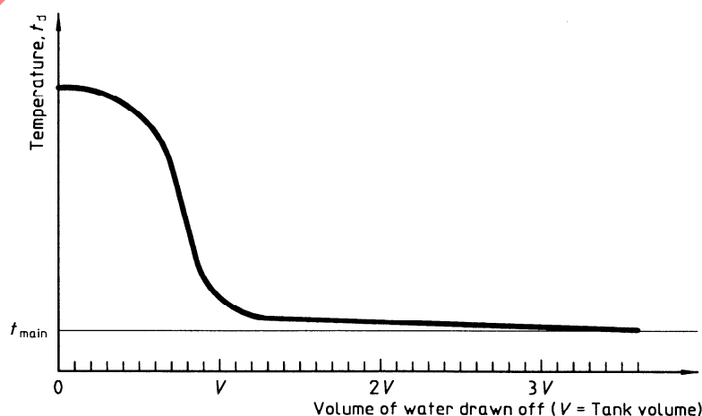
Figure 2 — Draw-off temperature profile
