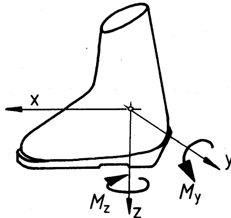
Figure 1 — Definition of the torques M_z and M_y
