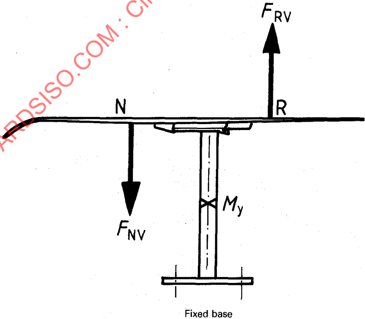
Figure 5 — Application of two equal forces F_{NV} and F_{RV} and measurement of M_{y, \max}
