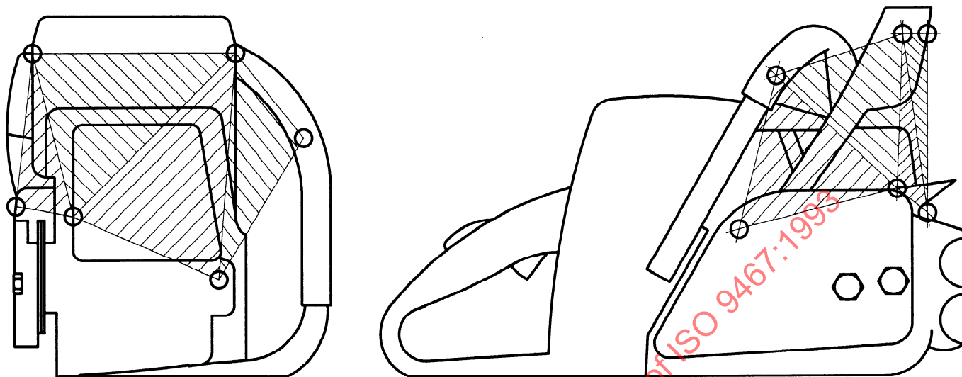
Figure 1 — Chain-saw with contact planes
