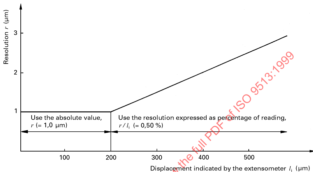
Figure B.1 — Resolution of a class 1 extensometer
